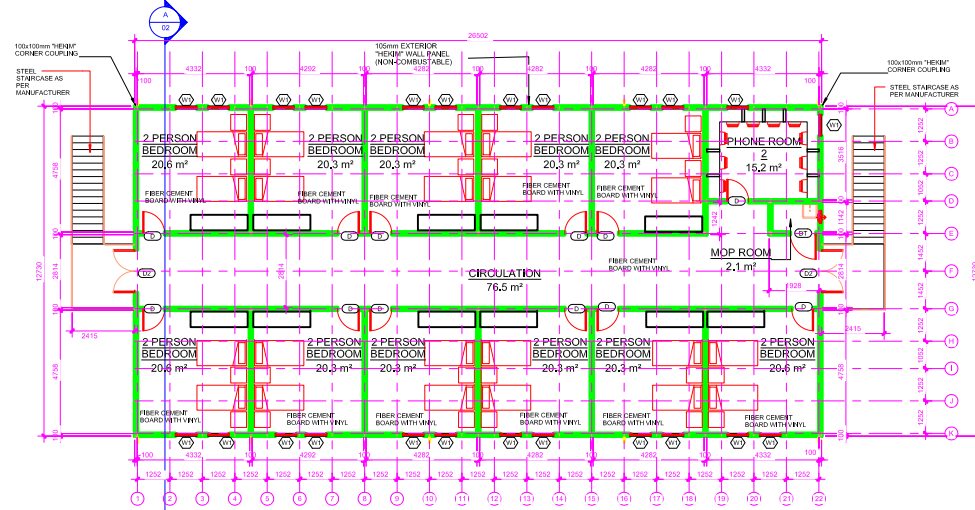
20-GROUND FLOOR PLAN 1:100
